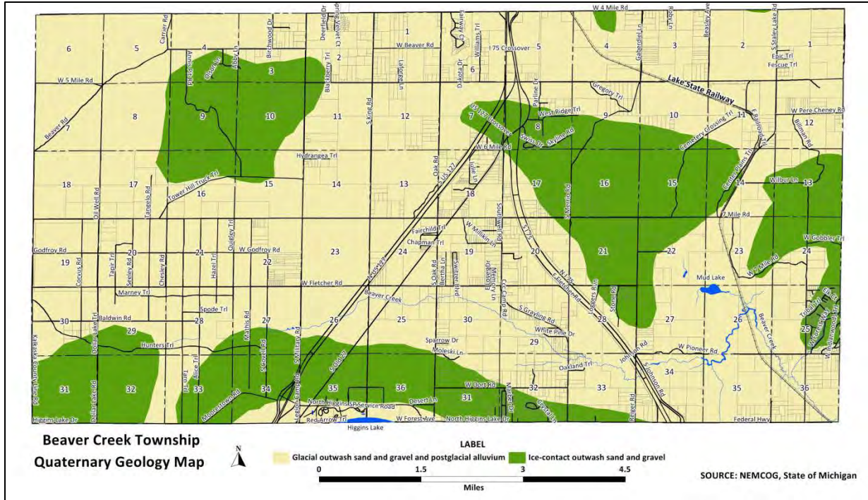
Figure 4.2 - Quaternary Geology Map, Beaver Creek Township
